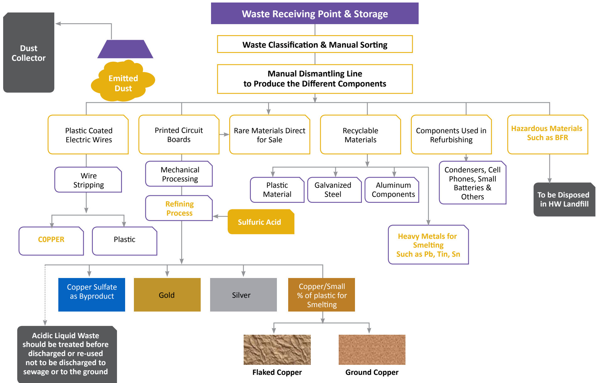
Figure 2: Process Flow Diagram of the Fractions Processing
